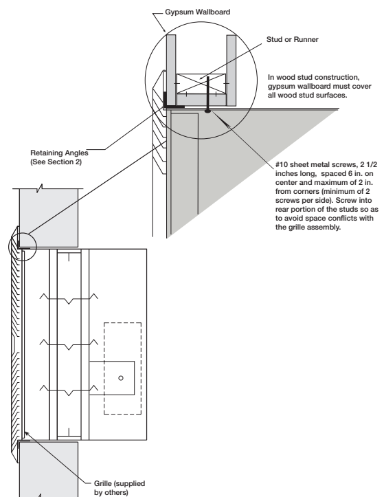
Figure 2 - Wood Stud
