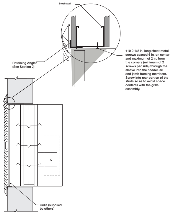
Figure 1 - Metal Stud
