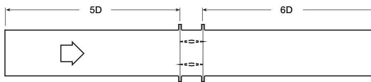
AMCA Figure 5.3
